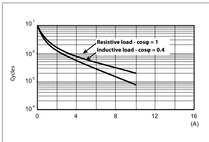
F 40.5 - Electrical life (AC) v contact current
